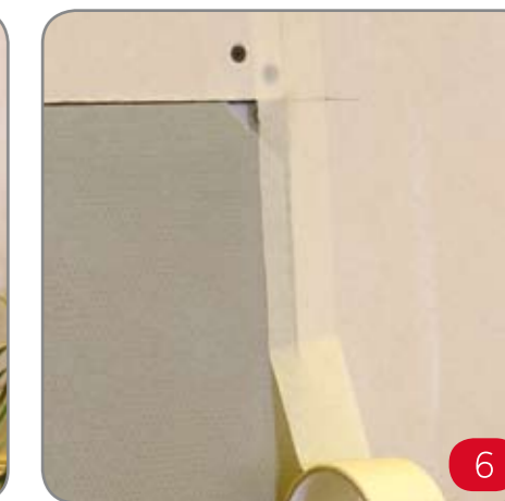
6 Apply joint tape, covering joint between panel and plasterboard. Perform final electrical/audio test.
