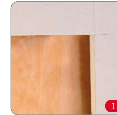
1 Create aperture using a sharp knife, making a series of shallow cuts. Add sound insulation into cavity.
